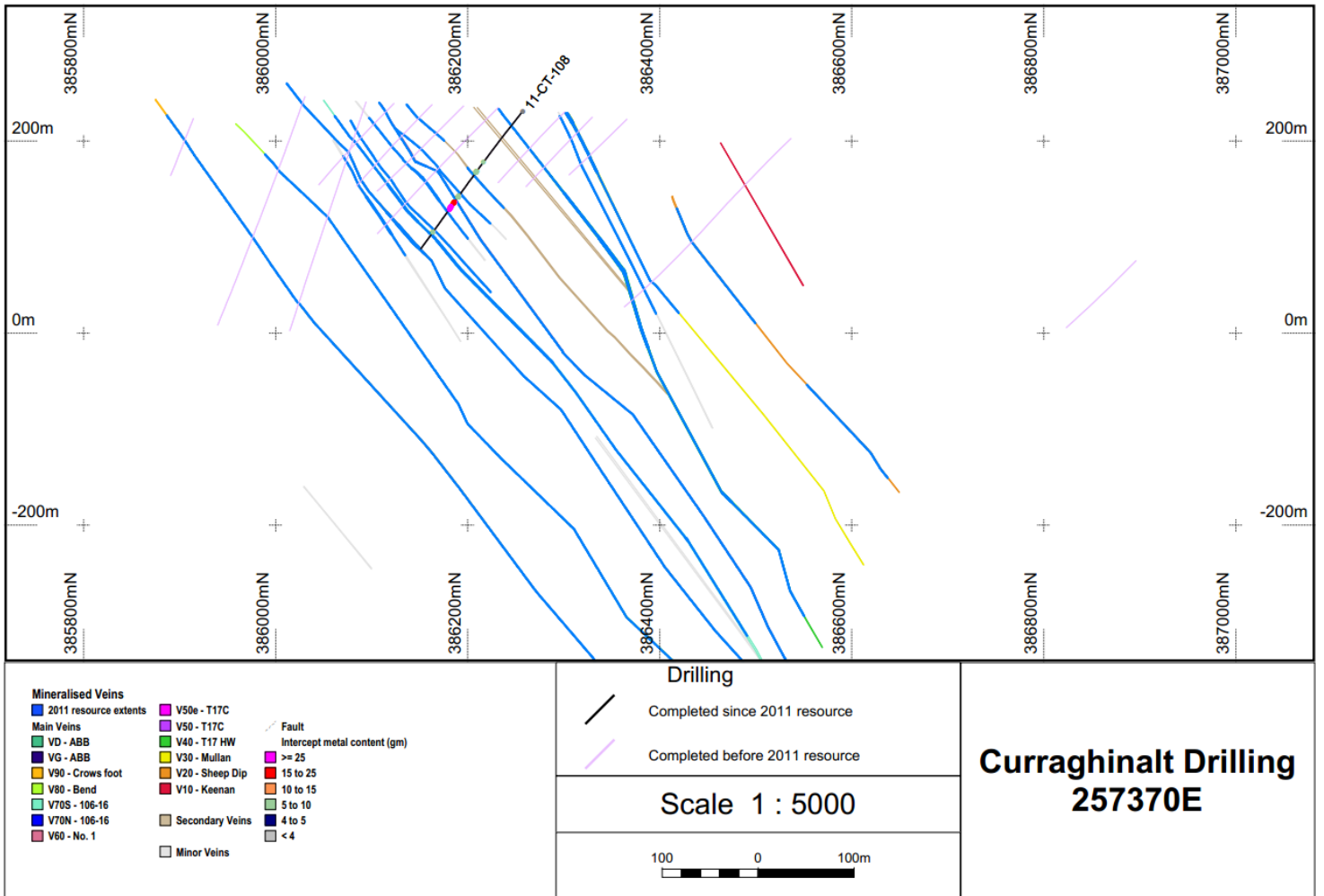
Figure 11: Representative Cross-Section 257370E
