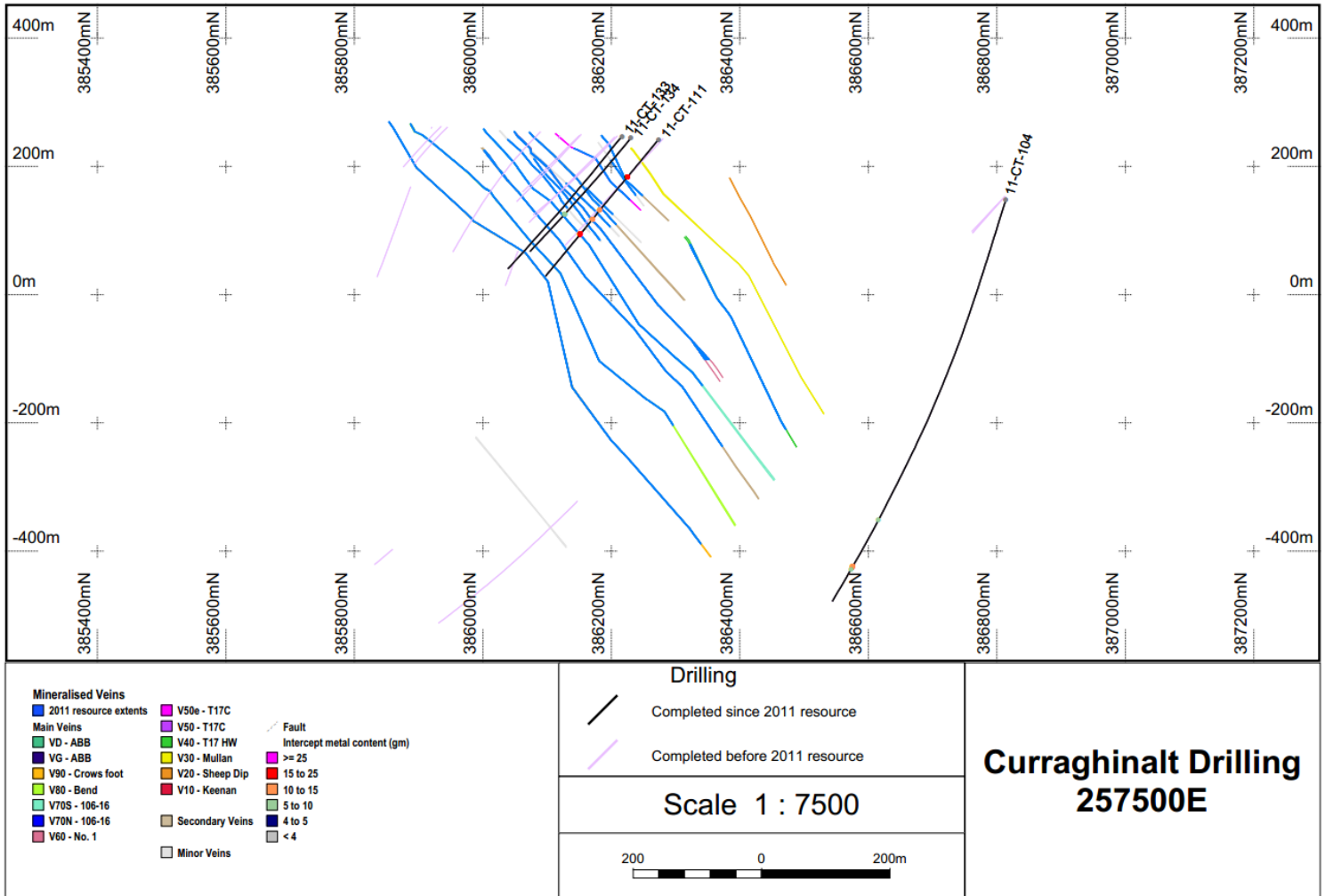
Figure 12: Representative Cross-Section 257500E
