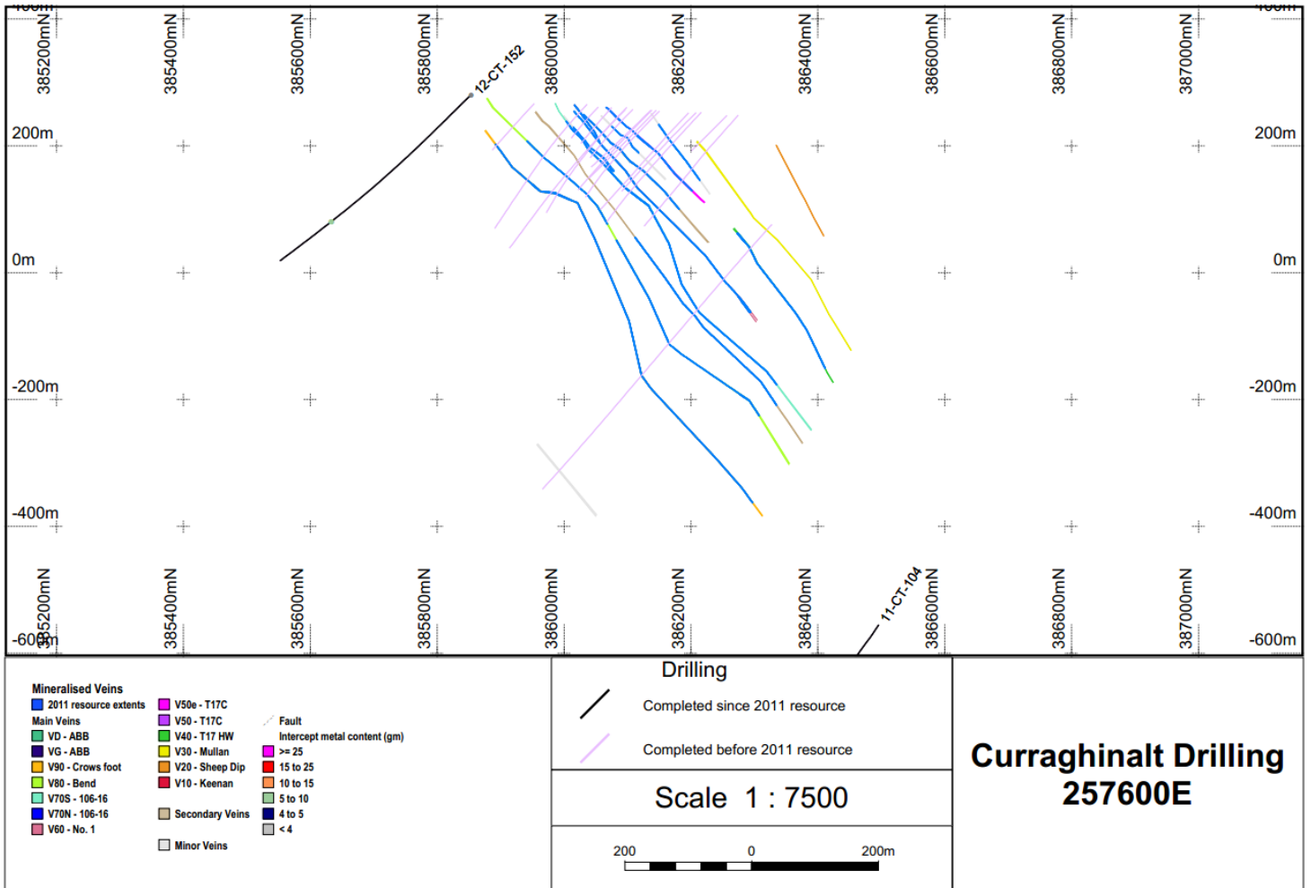
Figure 14: Representative Cross-Section 257600E
