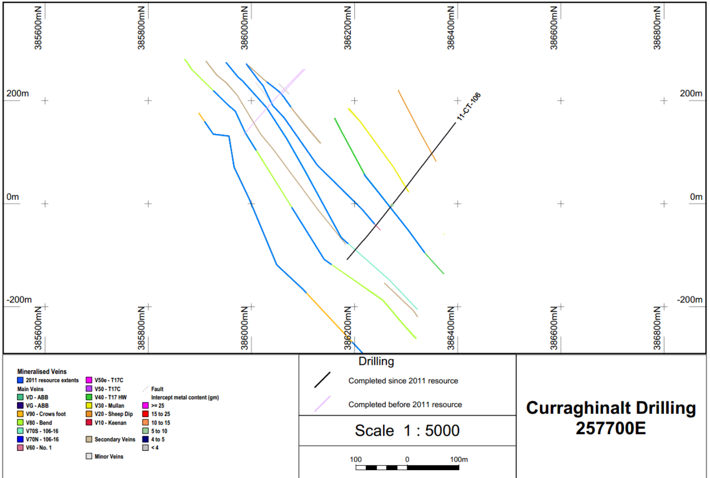
Figure 16: Representative Cross-Section 257700E
