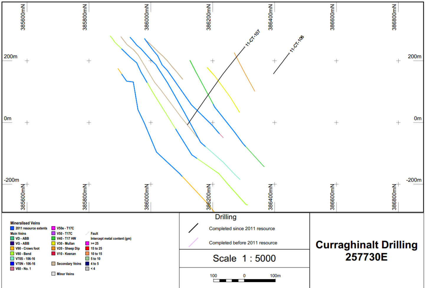
Figure 17: Representative Cross-Section 257730E
