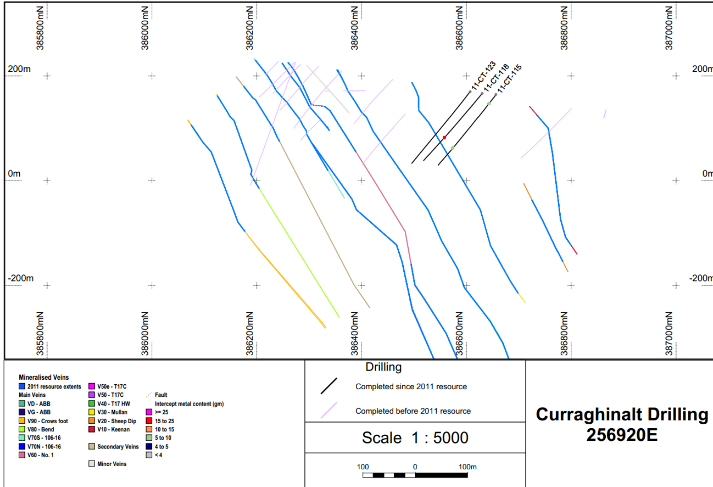
Figure 3: Representative Cross-Section 256920E
