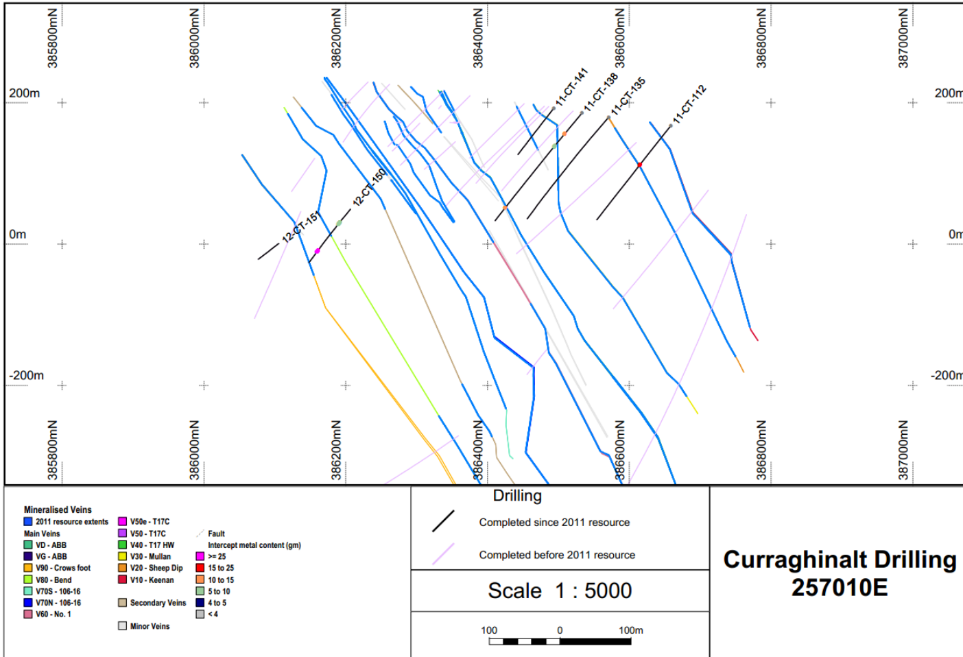
Figure 6: Representative Cross-Section 257010E
