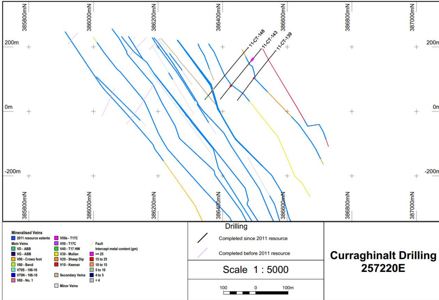
Figure 7: Representative Cross-Section 257220E
