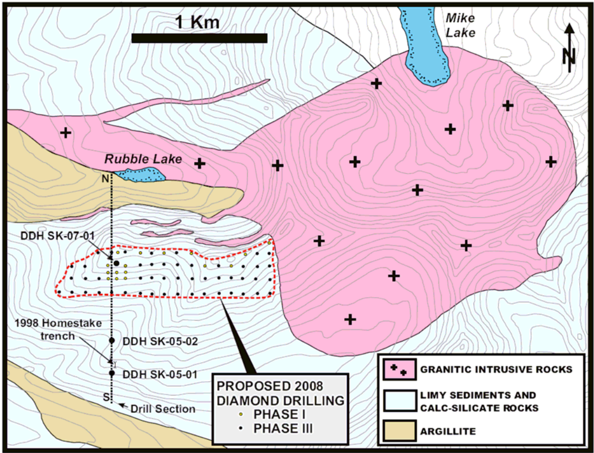
MAP 3: 2008 PROPOSED DIAMOND DRILLING PROGRAM – MIKE LAKE.
