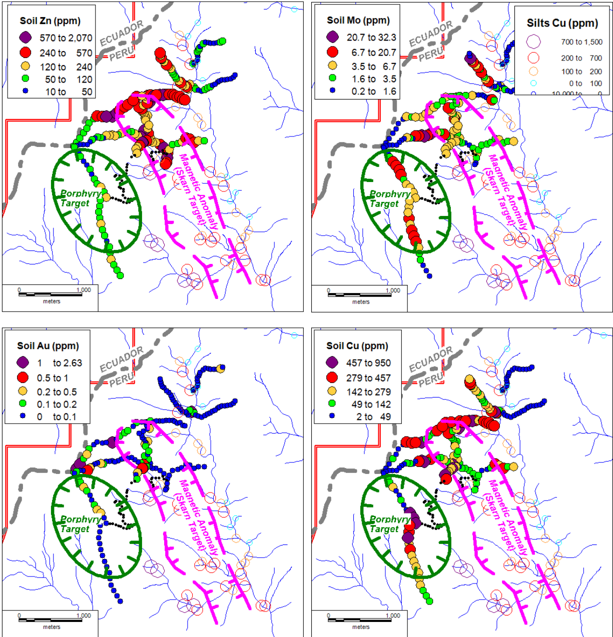
Figure 1: Soil Geochemical Results – Cobrecon Target (T4). These are preliminary results from an on-going program of ridge soil sampling. The small black dots are from lines that are pending results. In 2011 the work will continue to completely cover the area of magnetic high anomalies, outlined in magenta, as well as a magnetic low coincident with anomalous soil geochemistry, outlined in green.
