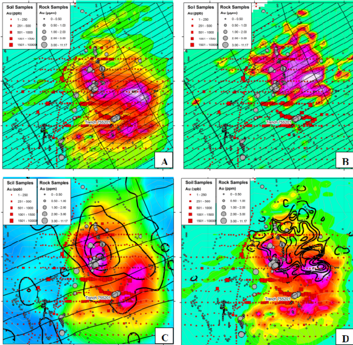
Figure 1. 2010 Airborne magnetic (Figure 1A) and electromagnetic (Figure 1B) survey results for the Lucero Target including flight lines (50 metre spacing) and surface rock and soil geochemistry. 2009 AeroTEM gridded magnetic anomaly map with EM anomaly contours (Figure 1C) and the gridded magnetic anomaly map with EM anomaly contours from the 2010 survey (Figure 1D) are shown for comparison. In both surveys the magnetic anomaly is coincident with the electromagnetic anomaly.
