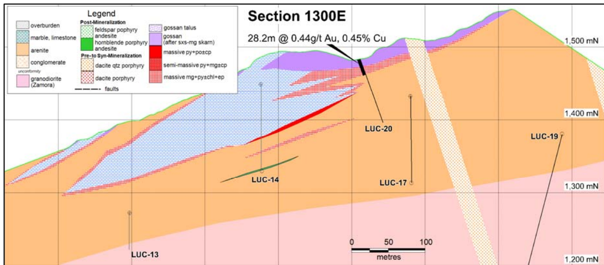
Figure 3: Section 1300 East including LUC-021 results
