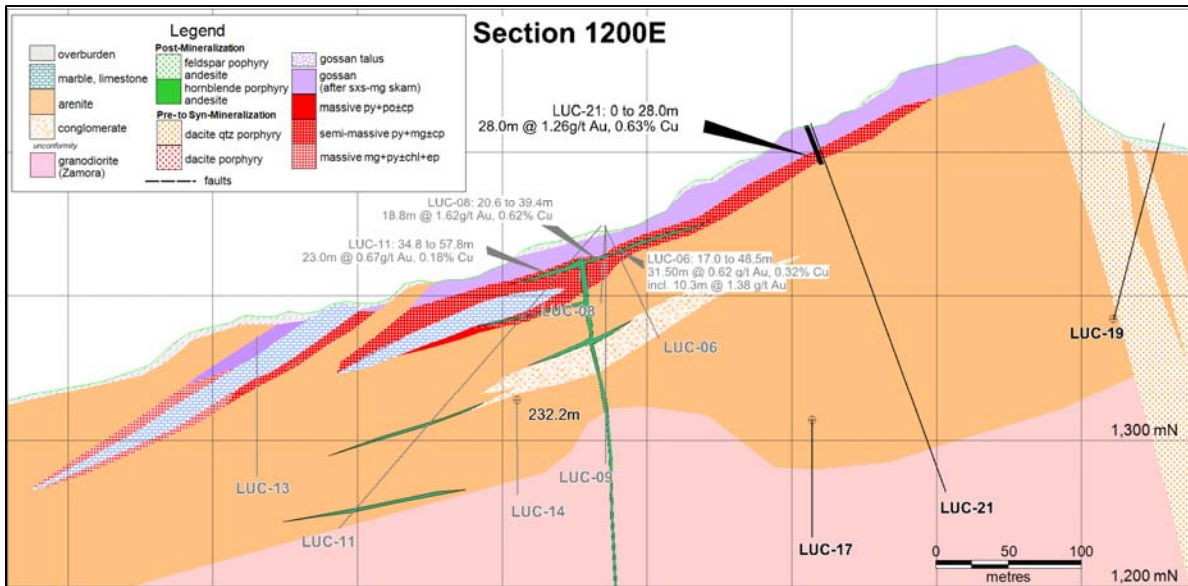
Figure 2: Section 1200 East including LUC-020 results
