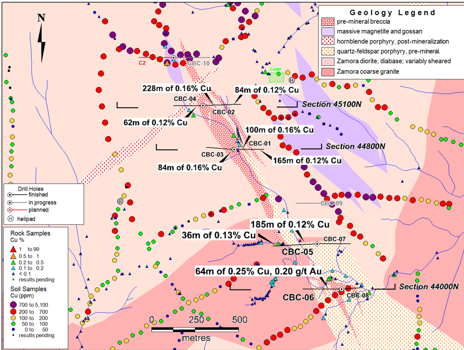
Figure 1: Cobrecon Drill Results Map. Significant intersections for holes CBC-05 and CBC-06.
