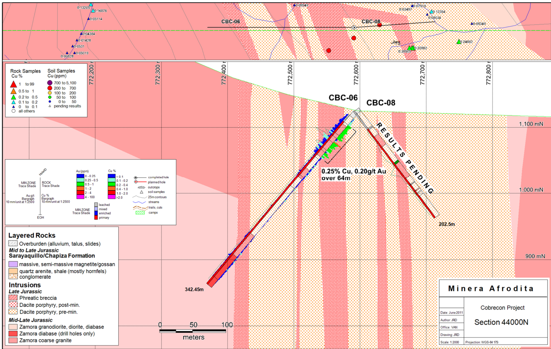
Figure 3. Cobrecon Cross Section 44000N, showing holes CBC-06 and CBC-08 (results pending).
