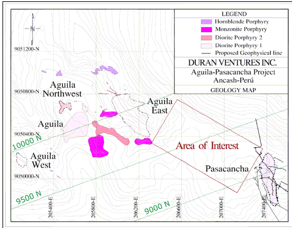
Figure 2 - Location of known intrusive bodies in the Aguila and Pasacancha areas. Dotted outlines indicate approximate limits in areas which have yet to be mapped in detail.
