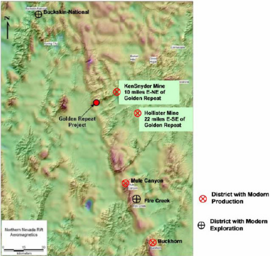
Figure 1 – Northern Nevada Rift Aeromagnetics
