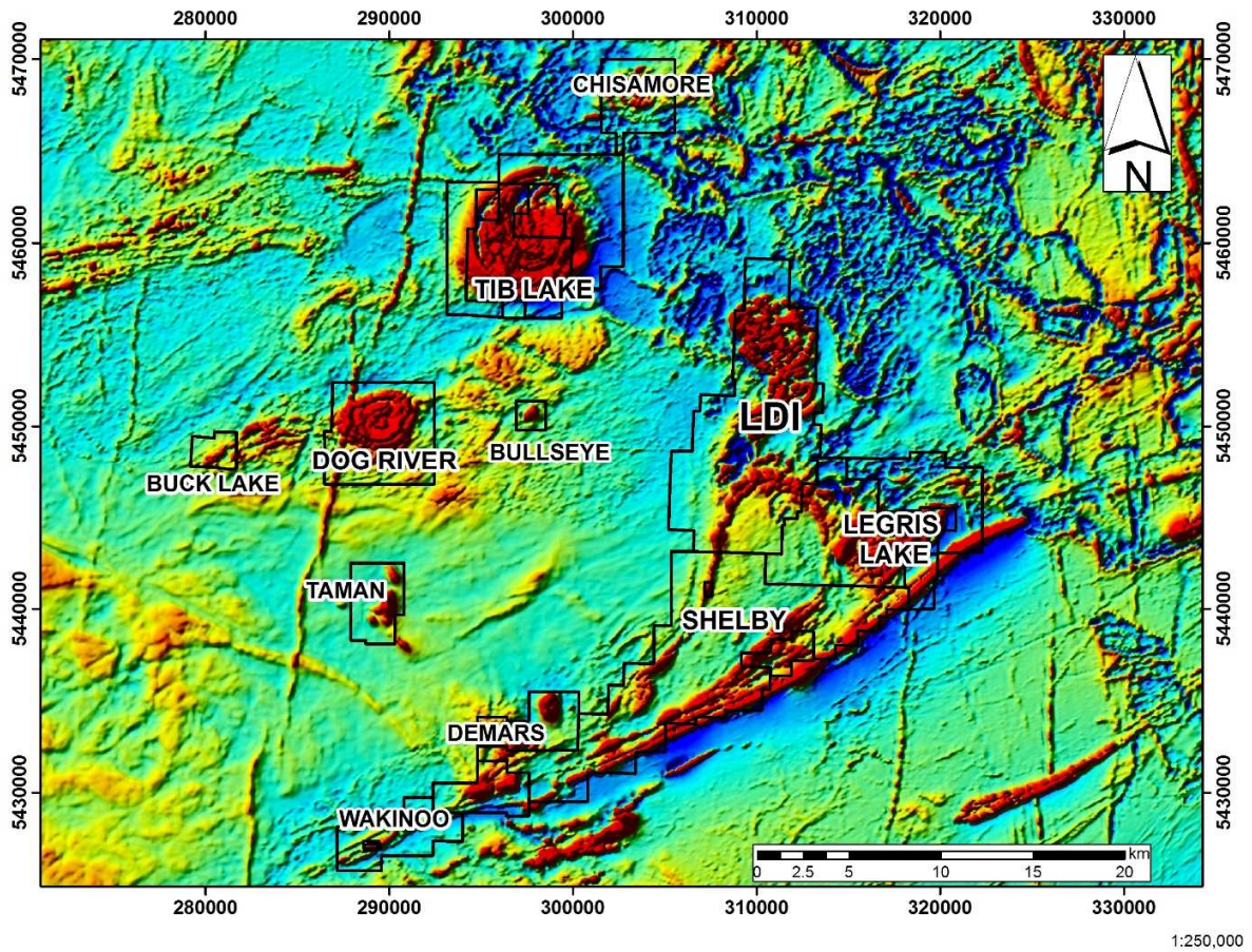
Figure 5. Location of the Company's Greenfields exploration properties (black outline polygons) with respect to the Lac des Iles Mine Property. The background image is a colour gradient total magnetic field map based principally on government airborne magnetic survey data. The grid coordinates reflect the NAD 83 datum and the UTM Zone 16N projection.
