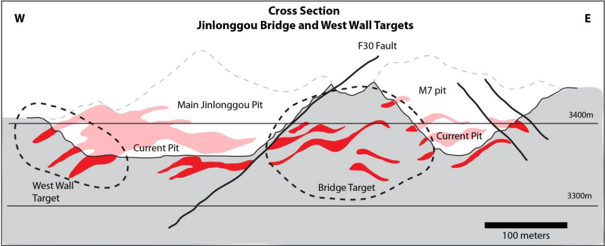
Figure 1: East-west cross section through the Jinlonggou Pit showing locations of the Bridge and West Wall target areas and schematic representations of gold mineralized zones
