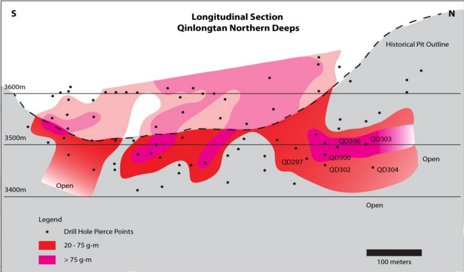
Figure 2: North-south longitudinal section through the Qinlongtan pit showing gold grade x thickness contours of previously mined material and in the Qinlongtan Northern Deep zone
