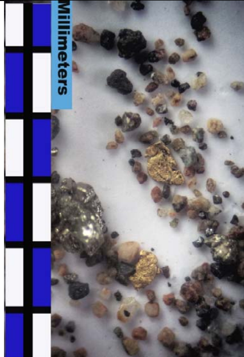
Optical photomicrograph of pan concentrate from Rio Blanco Suarez Fm polymictic conglomerate with agglomerate matrix sample: Au grains with predominantly sulphides, magnetite and quartz grains
