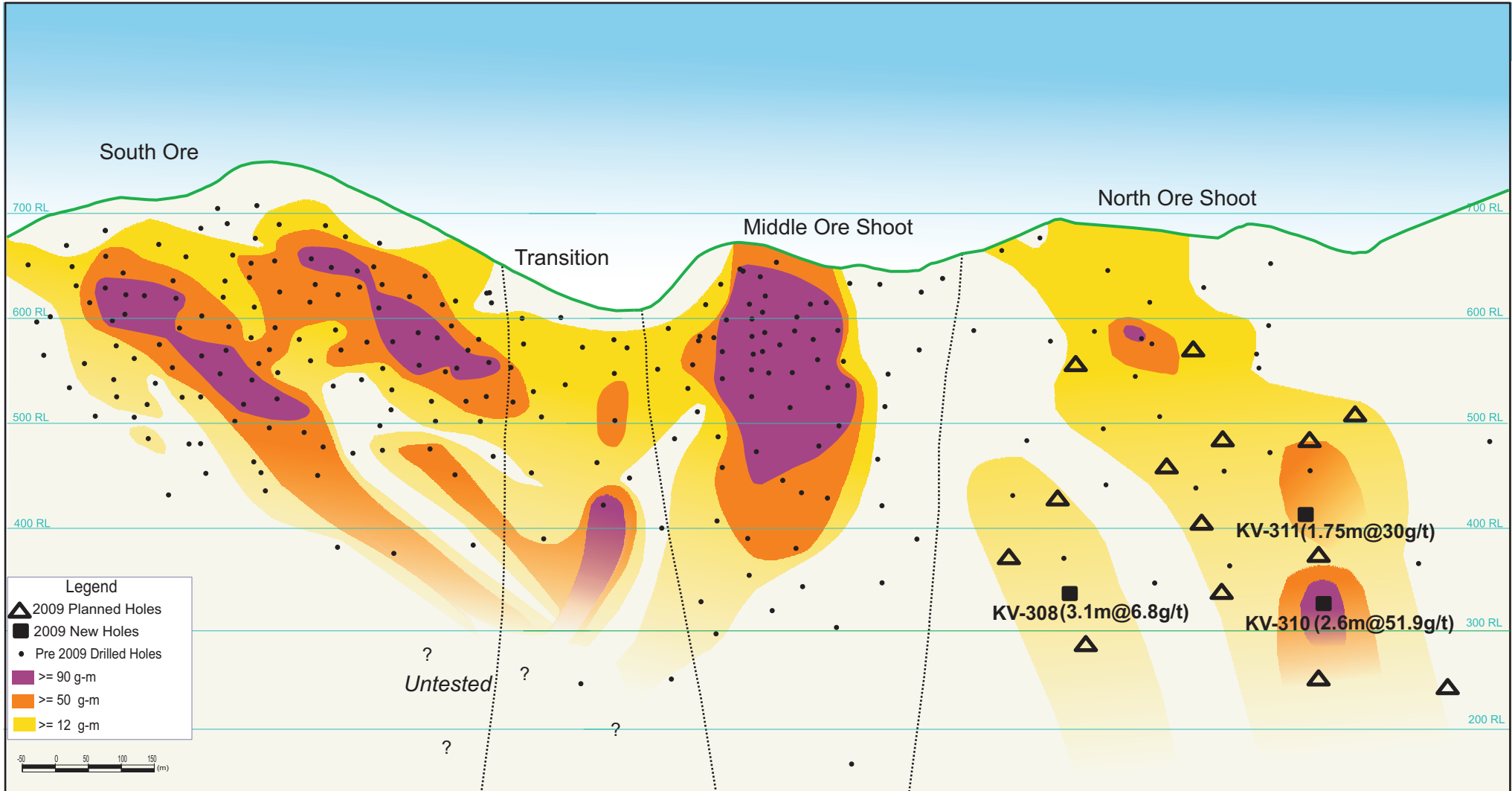
Figure 1 Efemçukuru North Ore Shoot Longitudinal Section Looking Southwest
