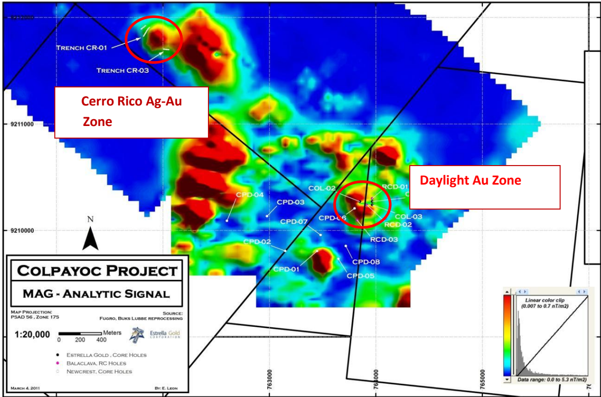
Figure 1. Colpayoc Project (partial area): ground magnetics data with drill holes and trench locations.
