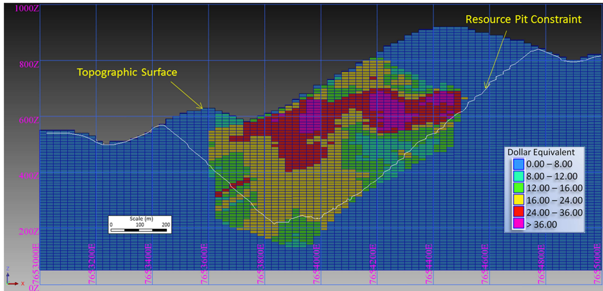
Figure 1. West-East Cross Section through the Centre of the Resource (Y = 4595180)
