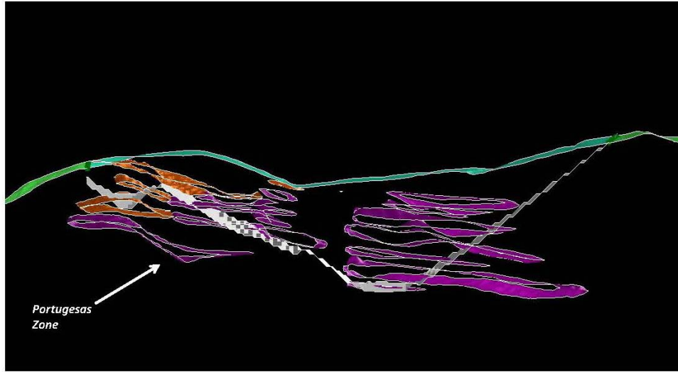
EAST WEST SECTION A-A' – 6526600 N Looking North
