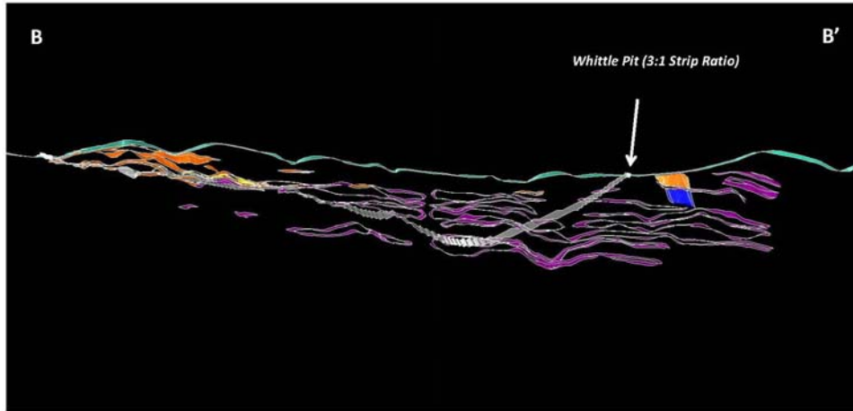
LONG SECTION B-B' Looking East
