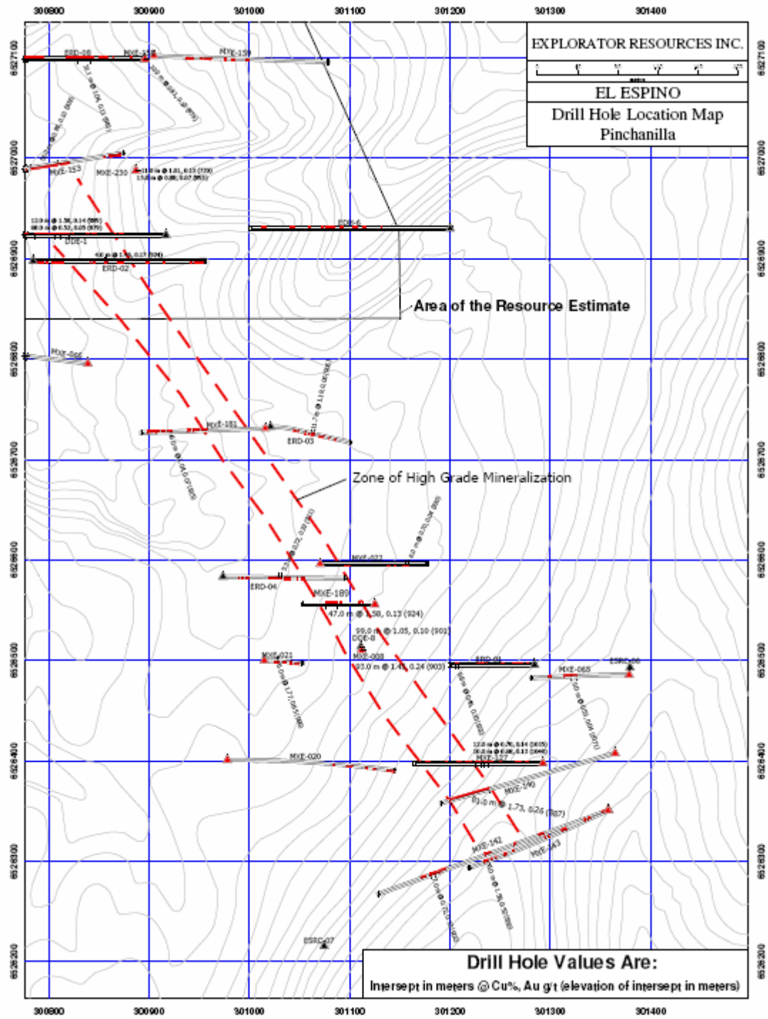
FIGURE 2 – PICHANILLA DRILL HOLES AND COPPER WORKINGS
