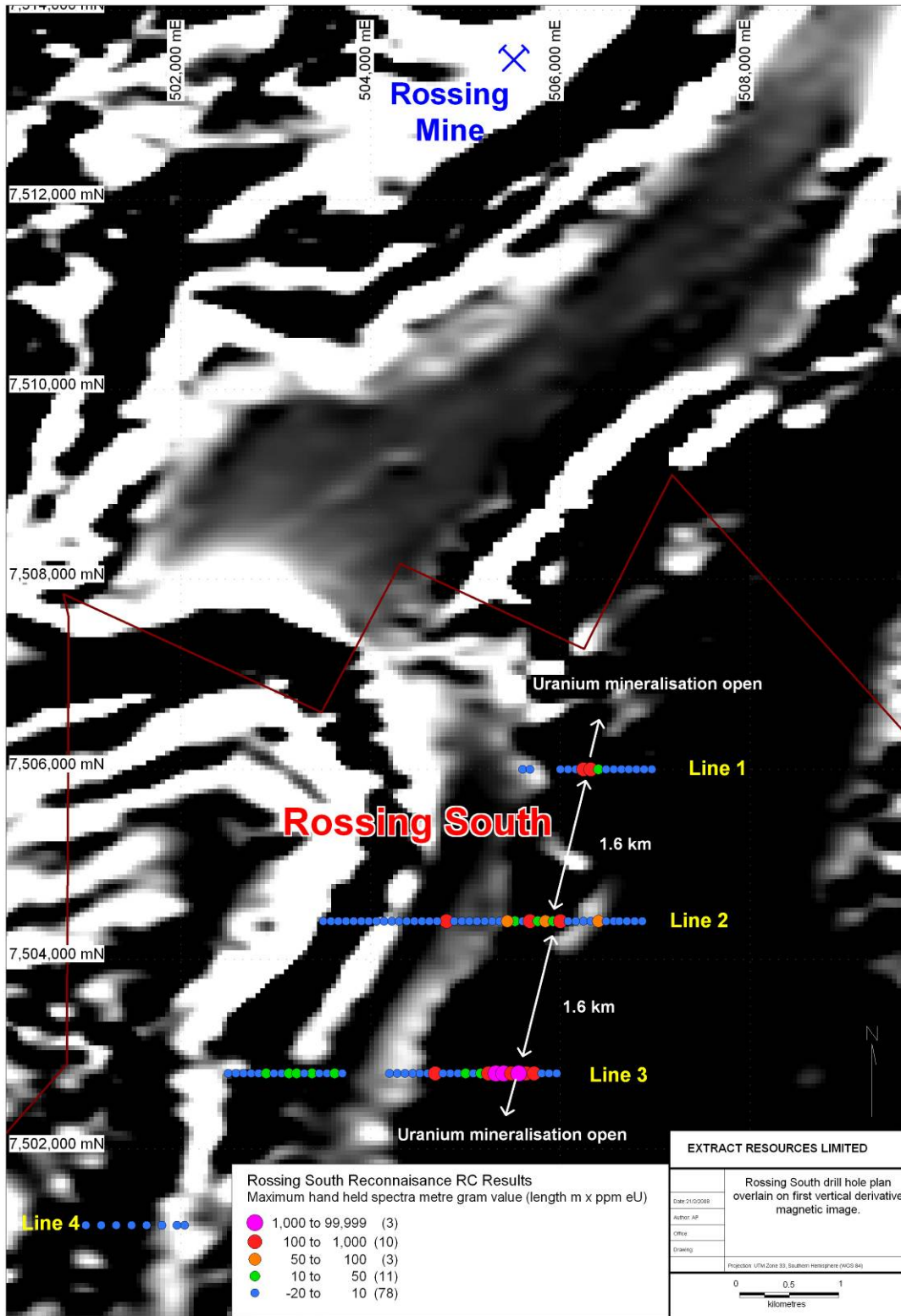
Figure 2: Rosing South drill hole location plan overlain on first vertical derivative magnetic data.
