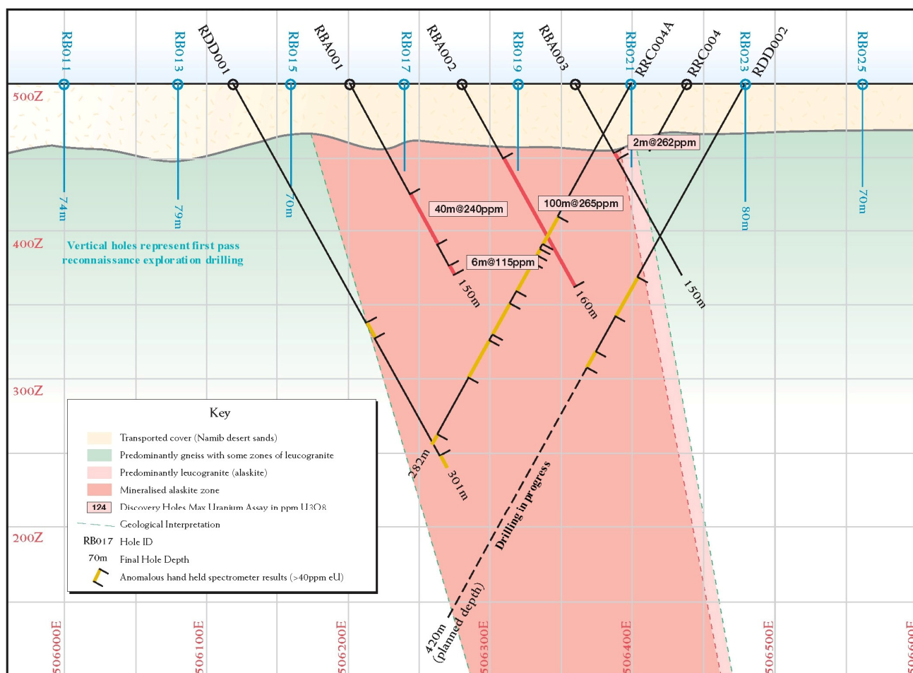
Figure 3: Rossing South drill hole section 7506000mN from Line 1. Projection UTM Zone 33, Southern Hemisphere (WGS 84).
