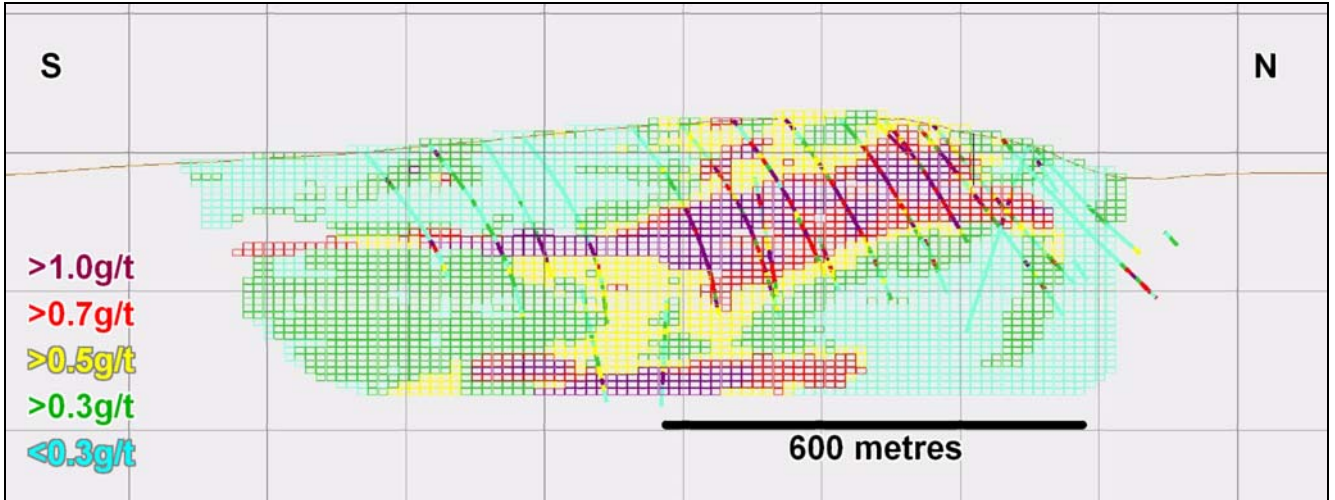
Figure 1: Resource model through Core Zone section 428925E illustrating the favourable geometry of the main Core Zone mineralization.
