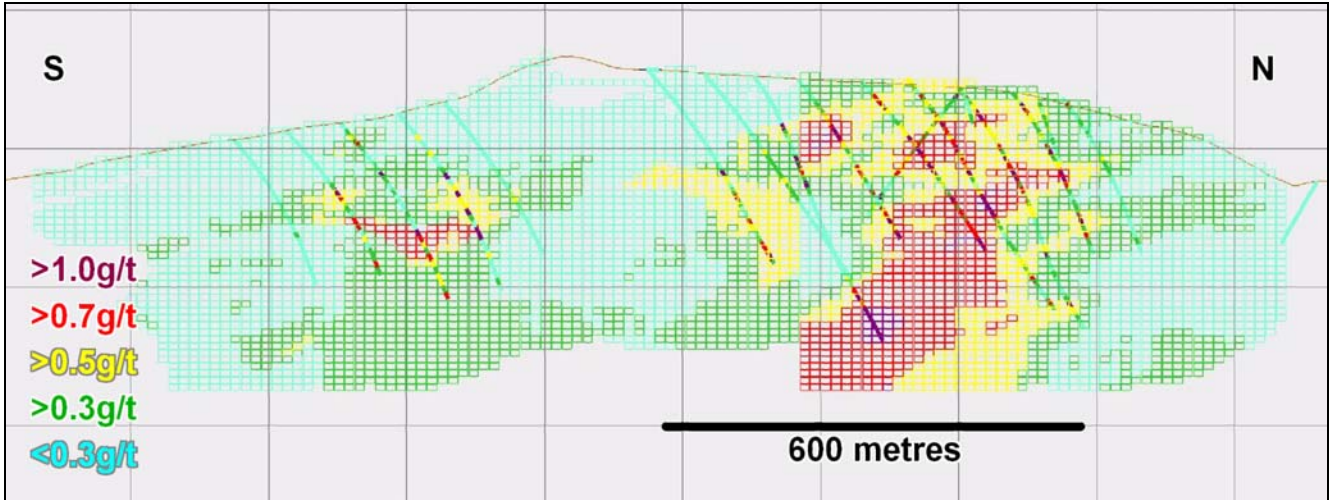
Figure 2: Resource model through Sunshine Zone section 429525E illustrating the geometry of the Sunshine Zone and the location of the Eastern Zone.
