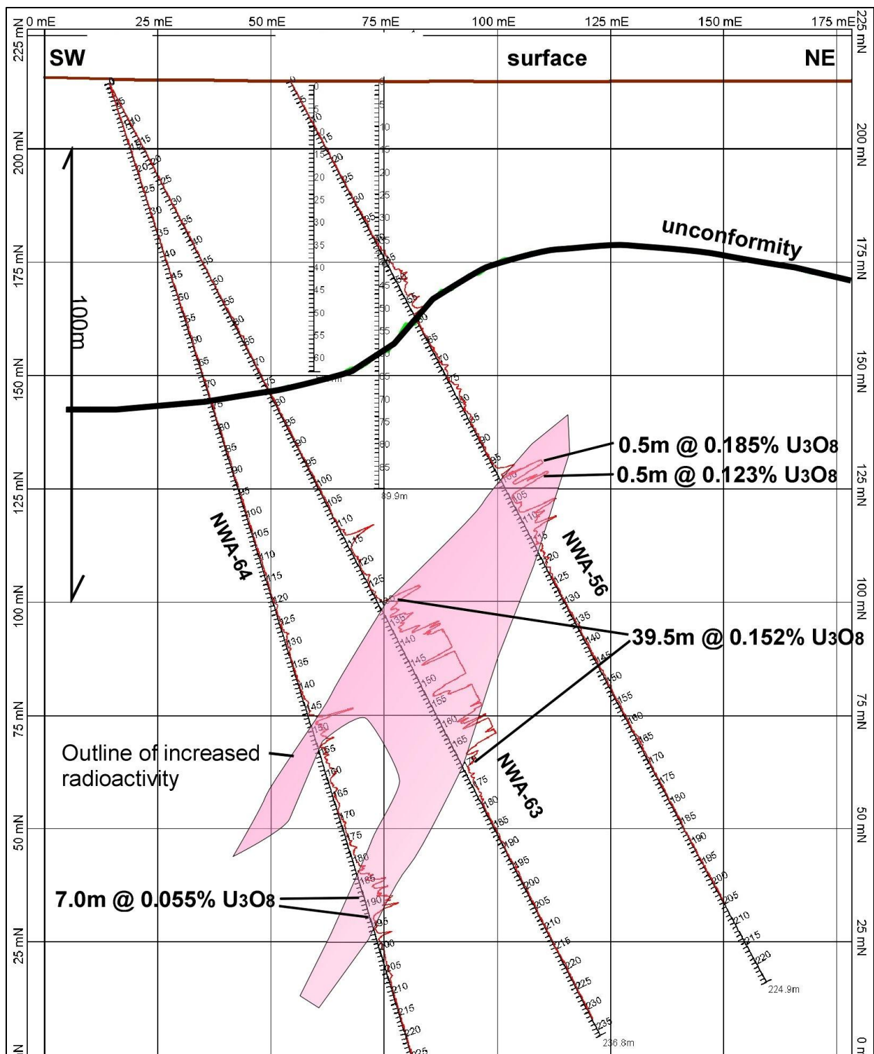
Figure 2: Cross-Section of NWA-56, 63 and 64. The grid is in 25m squares with the vertical showing elevation above sea-level. Hole NWA-63 returned local grades as high as 2.89% U 3 O 8 . The two short vertical holes are historic and drilled by Uranerz in 1978, narrowly missing the mineralization. Uranium mineralization was targeted at the unconformity, not in the basement at that time.
