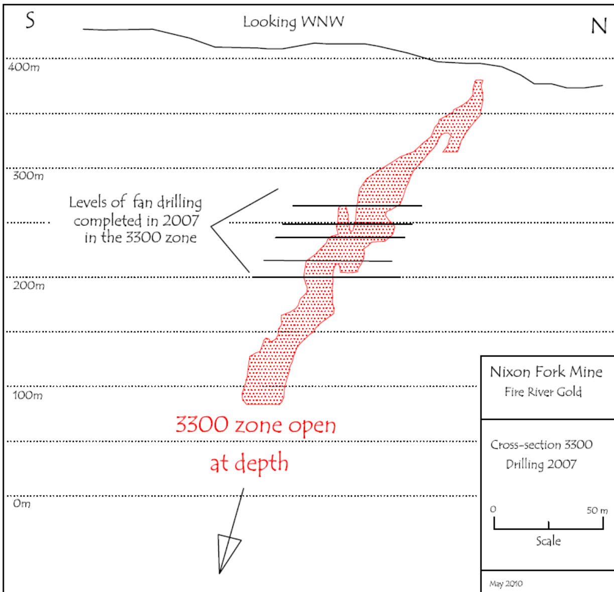
Figure 1. Cross-section through the 3300 gold zone in the Crystal decline, Nixon Fork.
