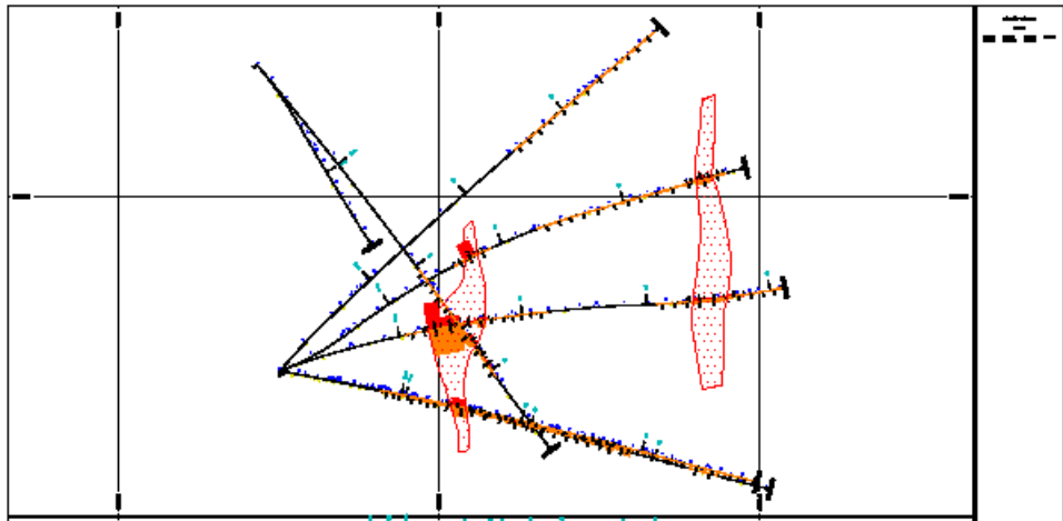
Figure 2. Typical underground fan drill station in the Crystal Mine, Nixon Fork decline showing mineralized zones.
