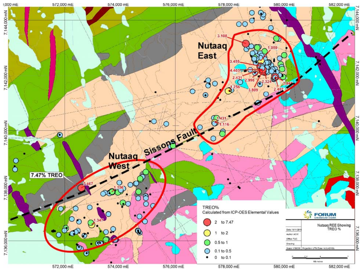
Figure 1: Geology of the Nutaaq Area with TREO% Samples. TREO samples with values greater than 1% are in red.
