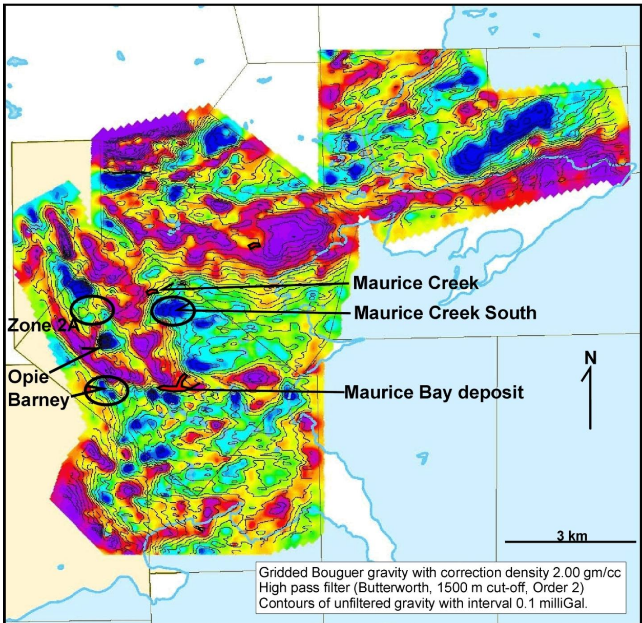
Figure 1: NW Athabasca Project Gravity Survey. The proposed 2012 fall drill targets on gravity lows (outlined in blue) are circled in black.
