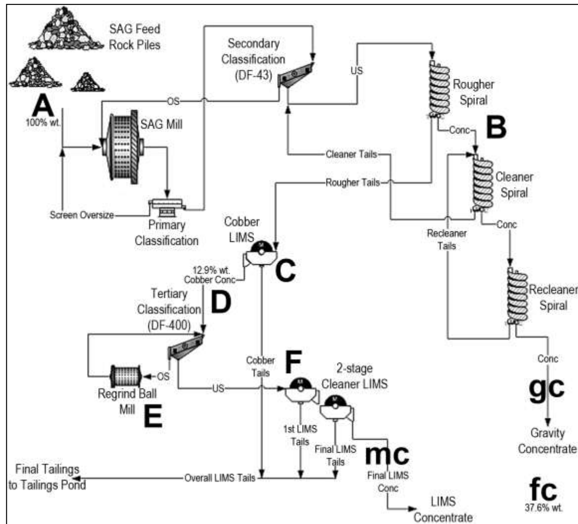
Figure 4 – Optimized Flowsheet
