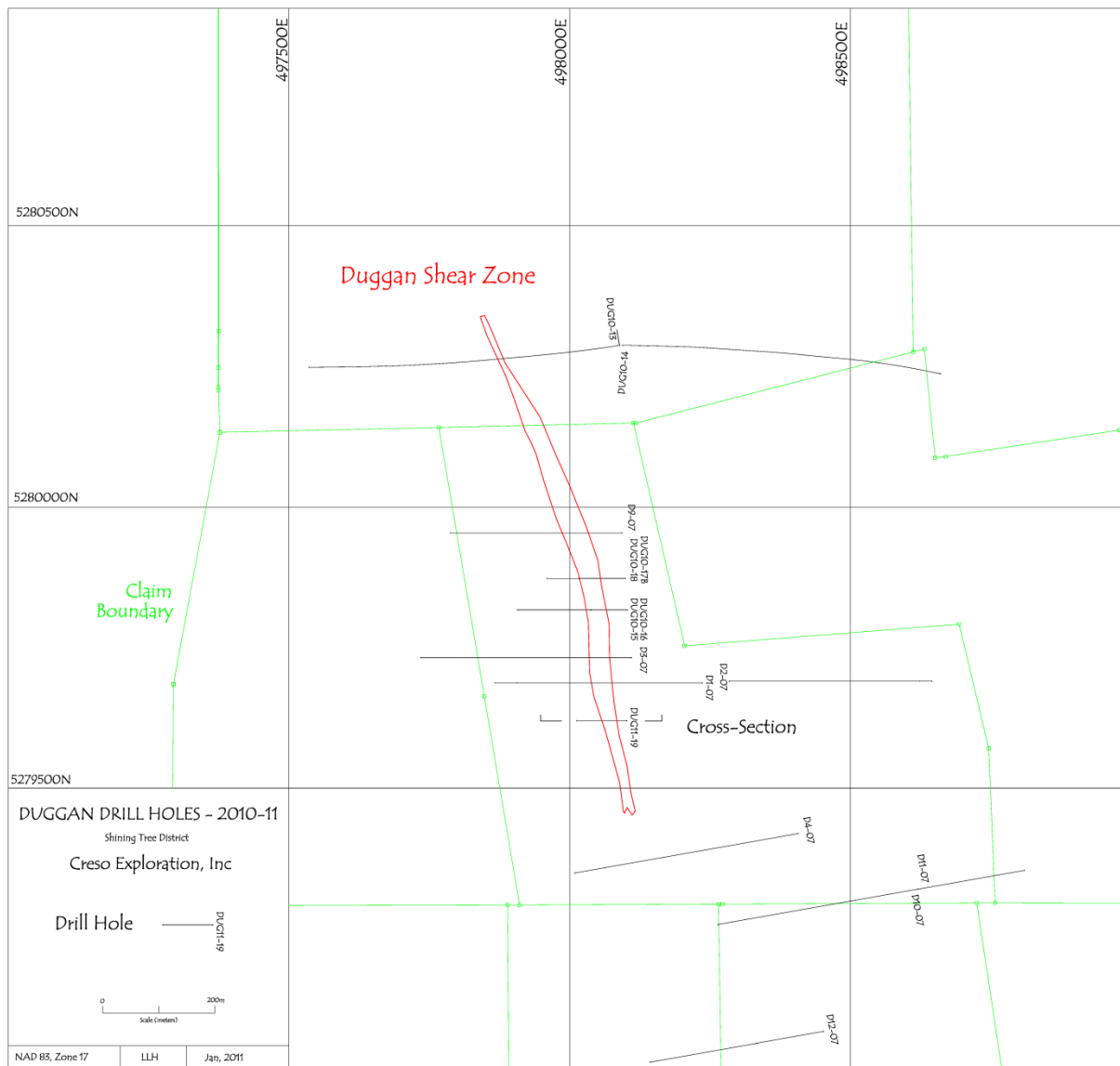
Figure 1. Drill Hole Locations at the Duggan Zone, Shining Tree District, Northeast Ontario.
