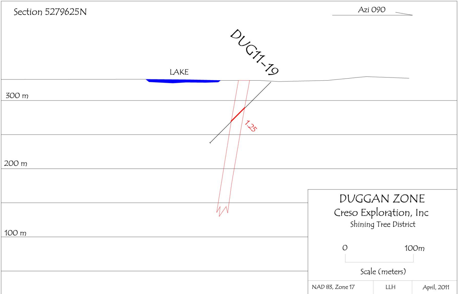
Figure 2. Cross-Section through DUG11-19 in the southern part of the Duggan Zone, Shining Tree District, Northeast Ontario.
