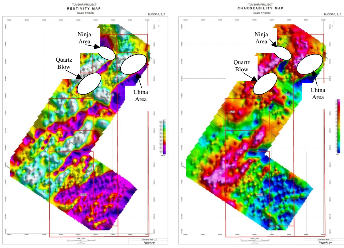
Figure 1: Gradient-Array survey with Resistivity and Chargeability results side-by-side.
