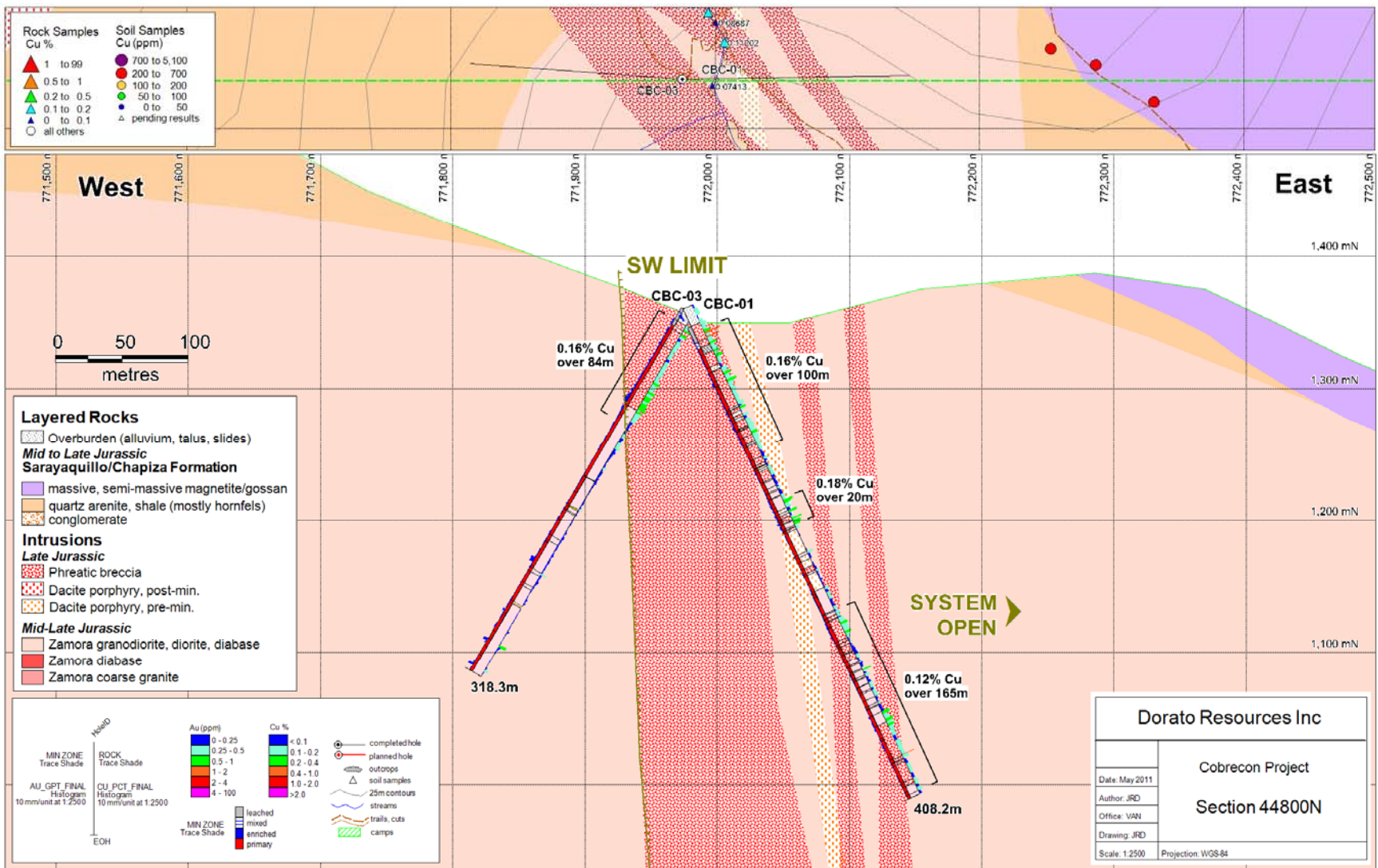
Figure 2. Cobrecon Cross Section 44800N, showing holes CBC-01 and CBC-03.
