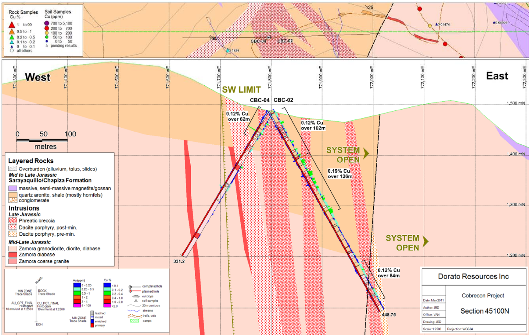
Figure 3. Cobrecon Cross Section 45100N, showing holes CBC-02 and CBC-04.
