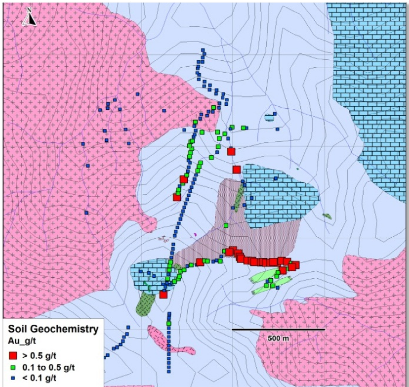
Figure 2: Gold-in-soil geochemistry
