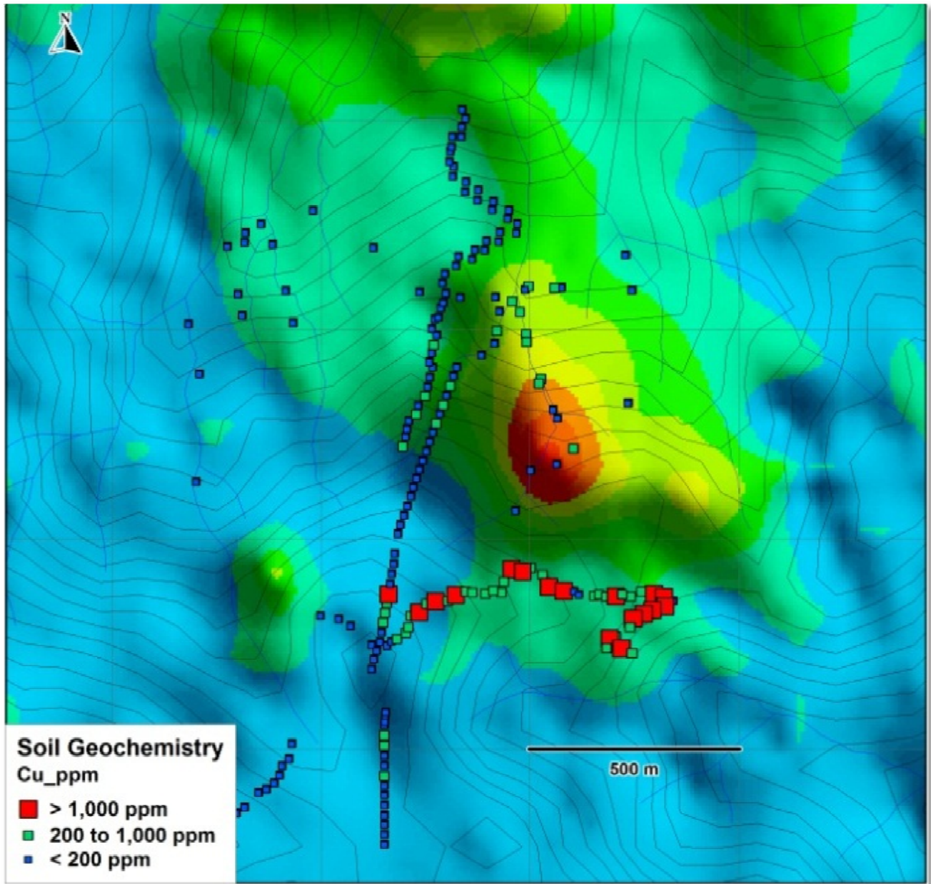
Figure 3: Copper-in-soil geochemistry
