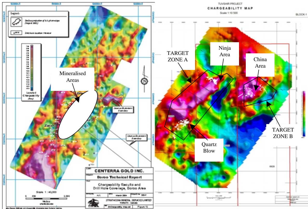
Figure 2: Centerra Gold's Boroo Chargeability results against Tuvshir's Chargeability results.
