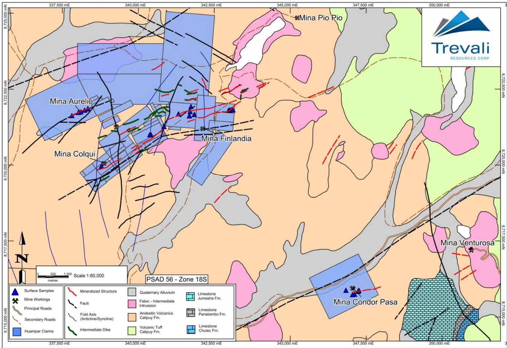
Figure 3: Simplified geological map showing the Huampar property and location of due diligence samples.
