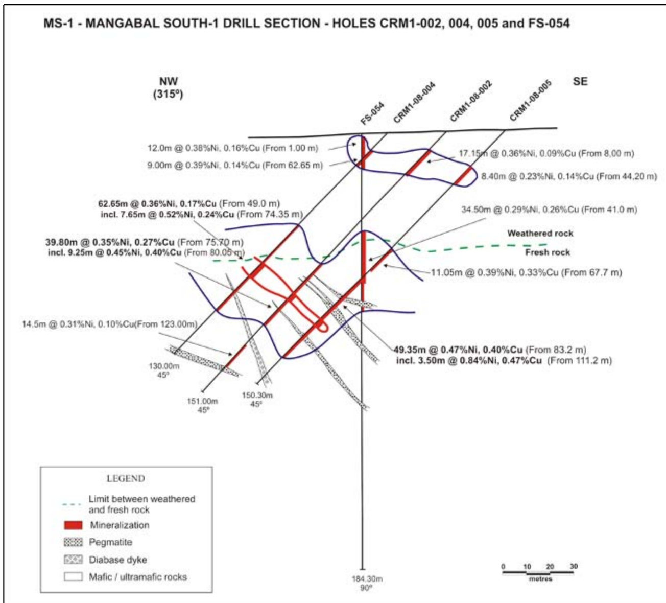
Figure 4: Section showing outline of mineralized zone at MS-1. Note the depth to the top of the zone is approximately 40 metres from surface and drilling along strike indicates it persists at shallow depths due to a shallow to sub-horizontal orientation for the zone.
