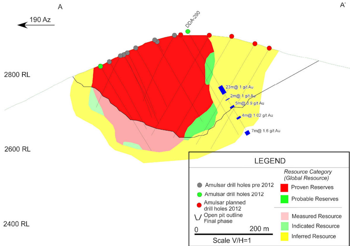
FIGURE 3. CROSS SECTION OF ERATO (SEE FIGURE 2) SHOWING RELEASED AND PLANNED 2012 DRILL HOLES AIMED AT CONVERTING INFERRED RESOURCES TO RESERVES
