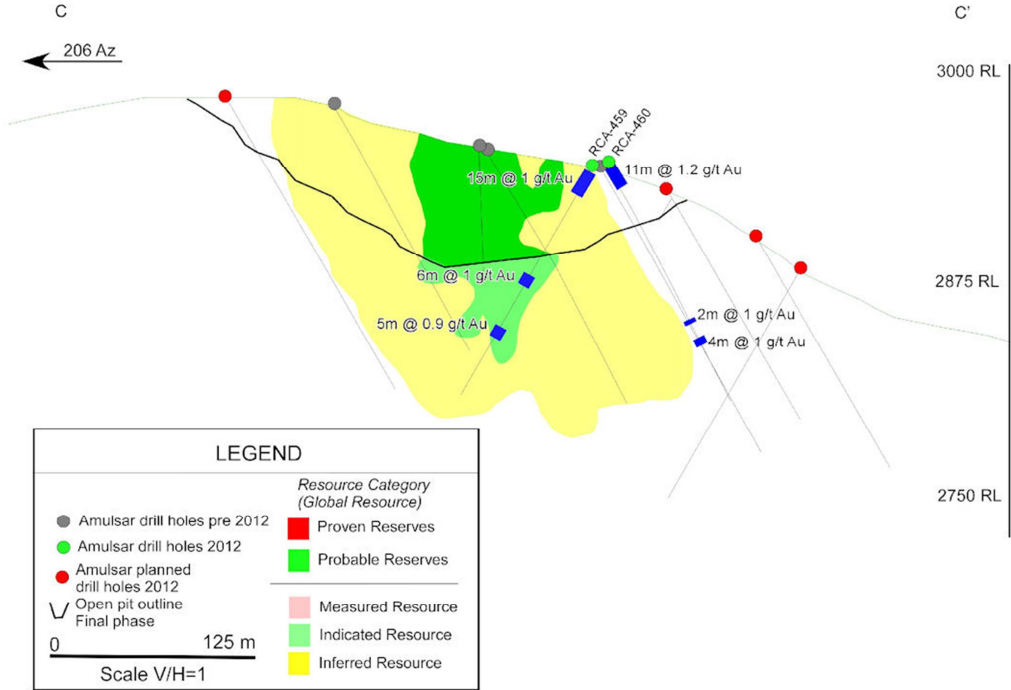
FIGURE 4. CROSS SECTION OF ARSHAK (SEE FIGURE 2) SHOWING RELEASED AND PLANNED 2012 DRILL HOLES AIMED AT CONVERTING INFERRED RESOURCES TO RESERVES
