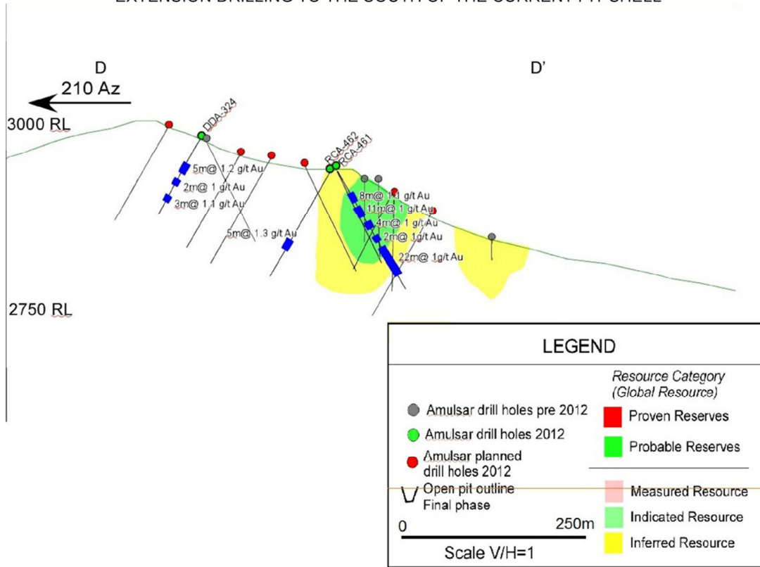
FIGURE 6. CROSS SECTION FROM ARSHAK (SEE FIGURE 2) ILLUSTRATING RESOURCE EXTENSION DRILLING TO THE SOUTH OF THE CURRENT PIT SHELL
