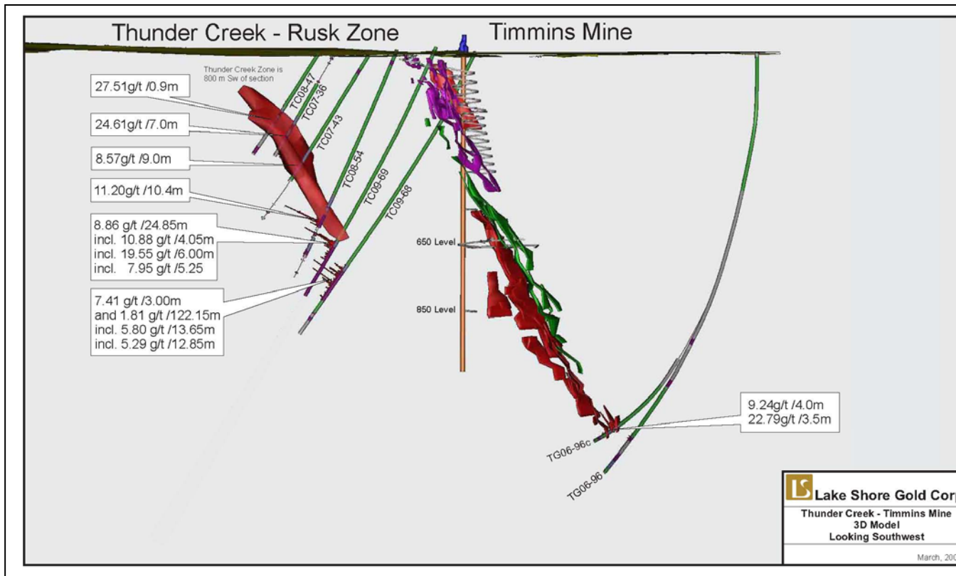
FIGURE 3. 3D VIEW
