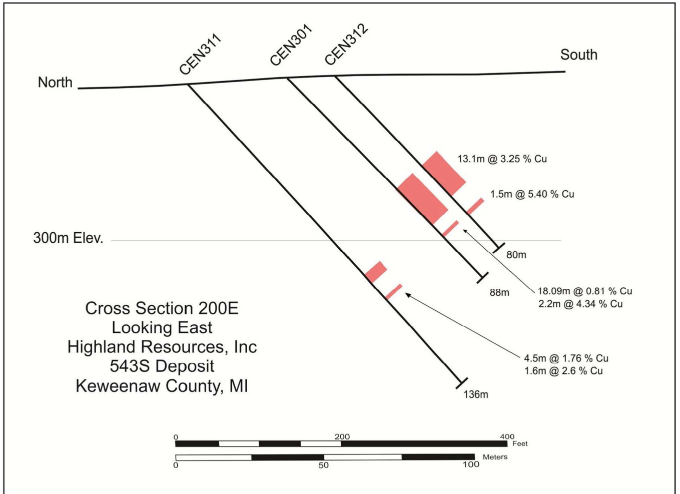
FIGURE 2. Cross section 200E, looking east, 543S deposit. Non-compliant historic drill holes are not shown. Holes CEN306 and 307 were inclined to the west from this section and are not shown.
