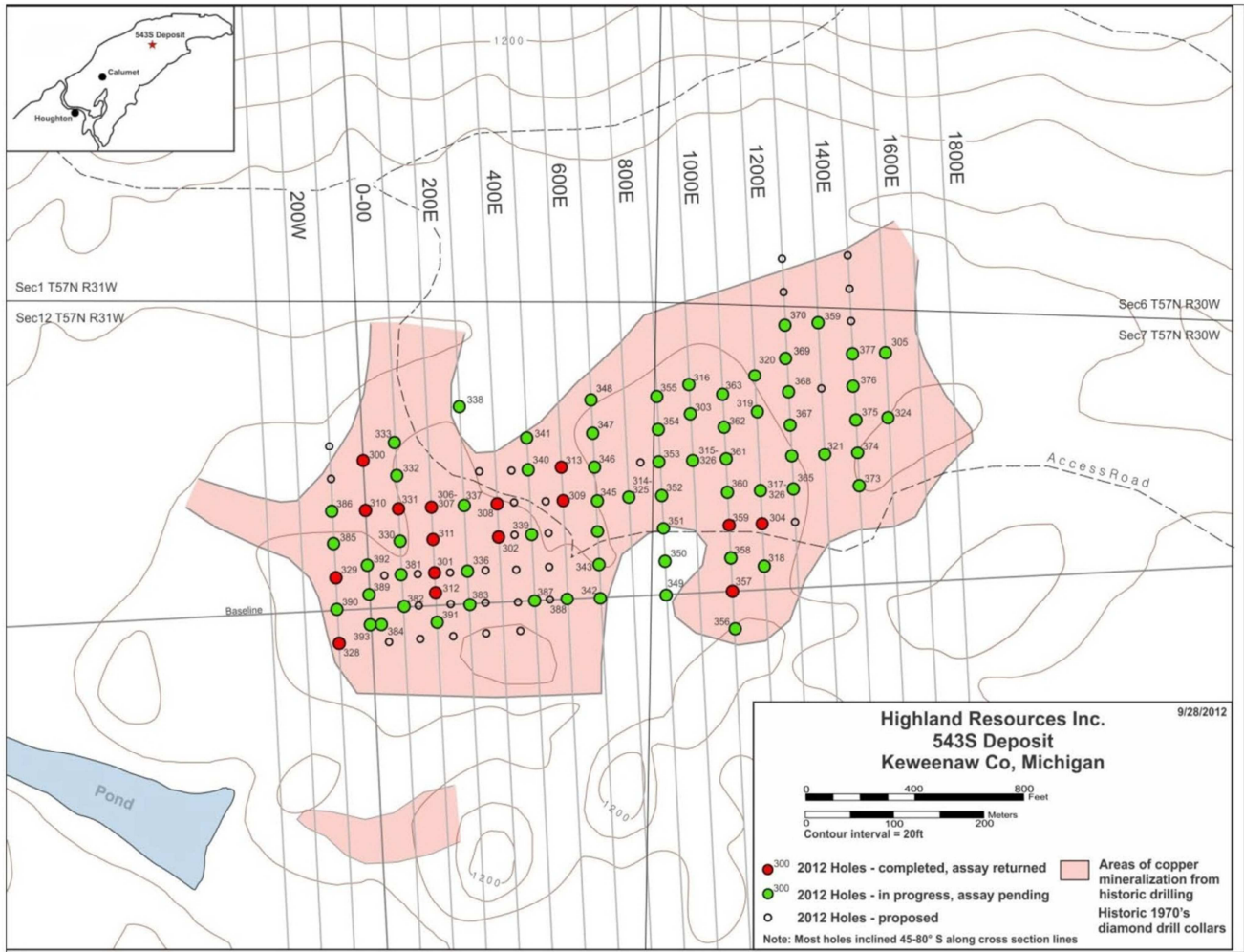
FIGURE 1. Drill hole locations at the 543S deposit. All holes inclined at 45-80 degrees to south on sections except holes CEN306 and 307 that are inclined to west.
