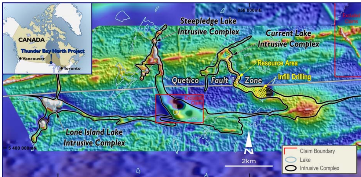
Figure 1. Aeromagnetic image showing the three Thunder Bay North intrusive complexes.
