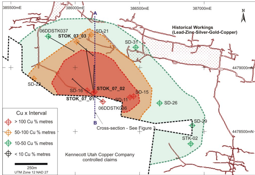
Figure 1. Plan view with interpreted copper x grade contours.
